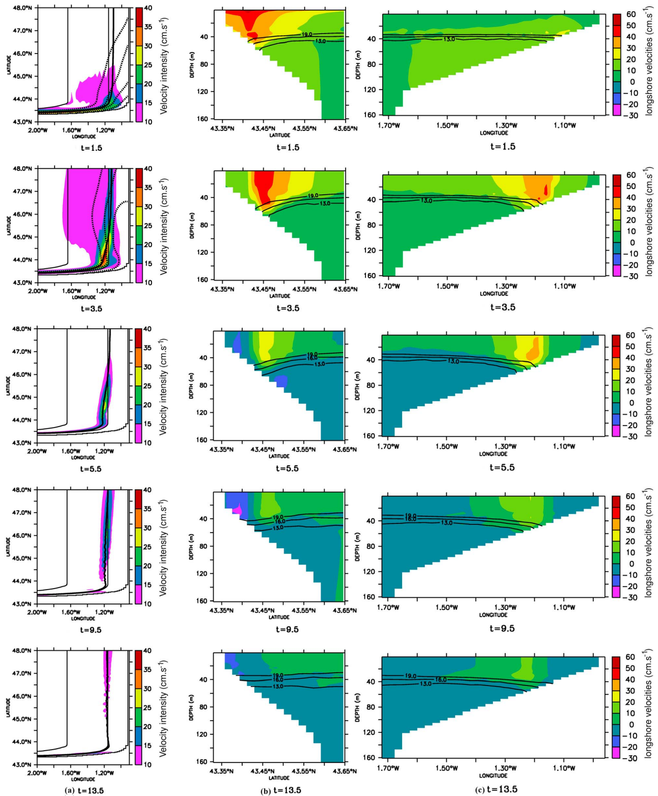
Figure 5. Results from the basic simulation (BC). (a) Depth-averaged velocities and location of the front (intersection between the isotherm 17°C and the bottom); solid lines: isobaths 0, 50, and 150; dashed lines: SSH isocontours from 4 cm to 10 cm in increments of 2 cm. (b) Vertical transect at 2°W of the zonal velocities and the superimposed isotherm. (c) Vertical transect at 44.5°N of the meridional velocities and superimposed isotherm for different times during simulation. Time is given in days.
