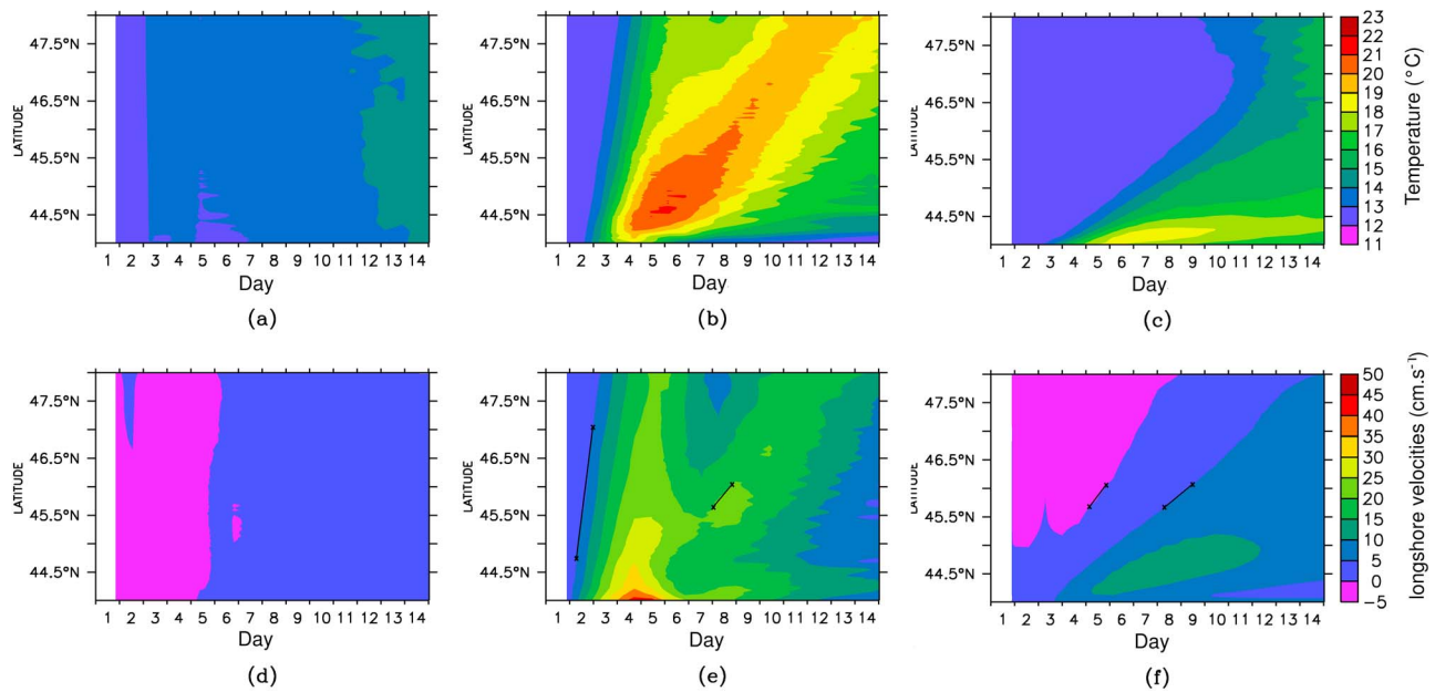
Figure 9. Bottom temperatures along the French coast on the 1.1°W transect from 44°N to 48°N at 46 m depth for (a) run SC1, (b) run SC2, and (c) run SC3. Maximum barotropic velocities over the shelf along the French coast for (d) run SC1, (e) run SC2, and (f) run SC3.
